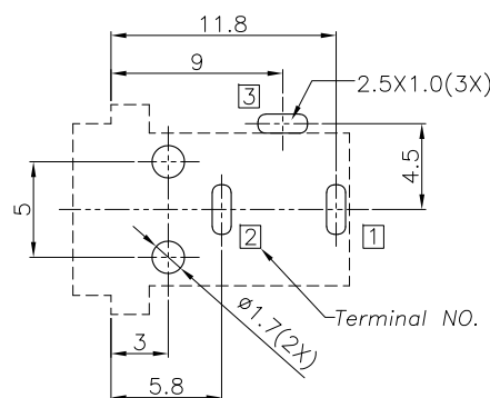
P.C.B. LAYOUT(TOLERANCE:±0.05) (BOTTOM VIEW)
