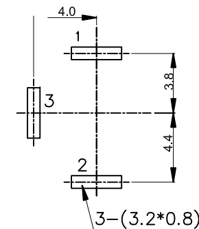
T:1.6 Dimensions of PC board holes Tolerance : ±0.1(Printed-sided view)
