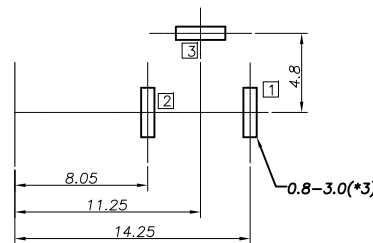
P. C. B. LAYOUT (COPPER-SIDED VIEW)
