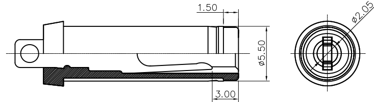
RECOMMENDED PLUG ø5.5 PLUG
