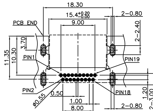
RECOMMEND PCB LAYOUT TOLERANCE: \pm 0.05 TOP VIEW
