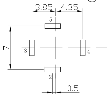
P. C. B LAYOUT
