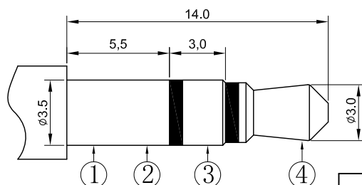
Ø3.50mm 3 POLE PLUG
