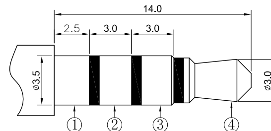
Ø3.50mm 4 POLE PLUG
