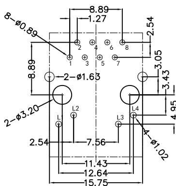
SUGGESTED PCB LAYOUY (TOP VIEW)
